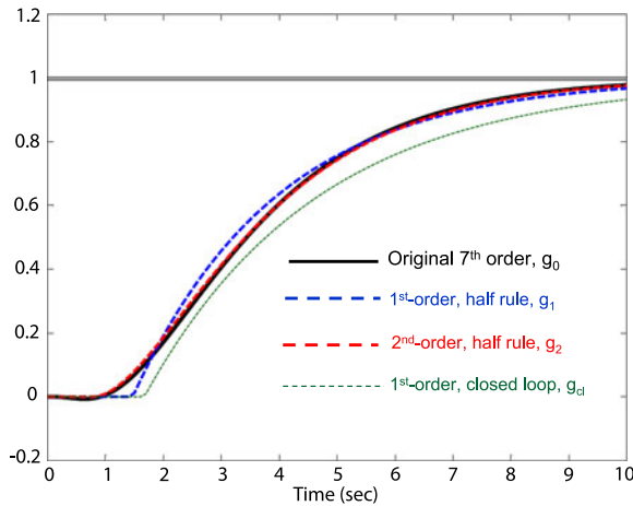
Fig. 5.5 Open-loop response to step change in input u for process E2, g_0(s) = \frac{(-0.3s+1)(0.08s+1)}{(2s+1)(1s+1)(0.4s+1)(0.2s+1)(0.05s+1)^3} (solid line), and comparison with various approximations
