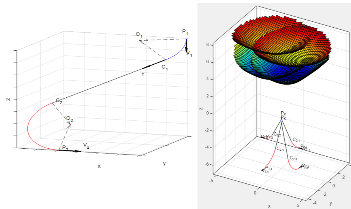
Figure 4: 3D Dubins path
