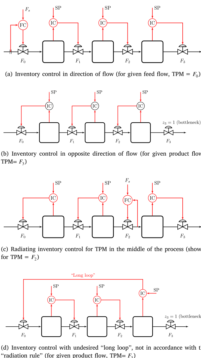
Fig. 35. Inventory control for units in series. Cases (a), (b) and (c) are in accordance with the “radiation rule”.
