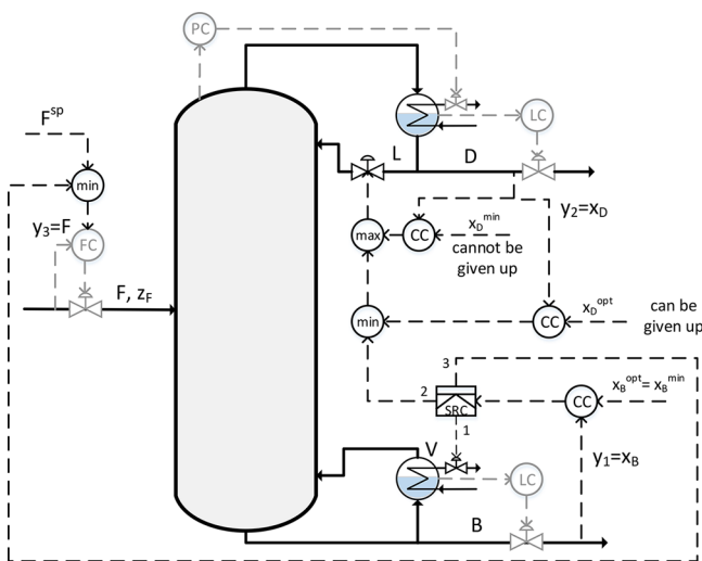
Figure 21. Alternative control structure for distillation column (all regions). This structure behaves differently from that in Figure 18 when maximizing throughput (region IV).
