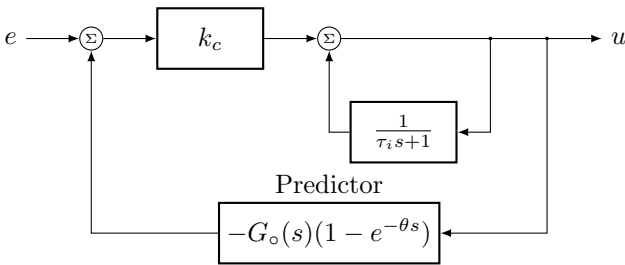
Fig. 2. Block diagram of the SP controller, K_{\text{SP}} , when K_o is a PI controller.
