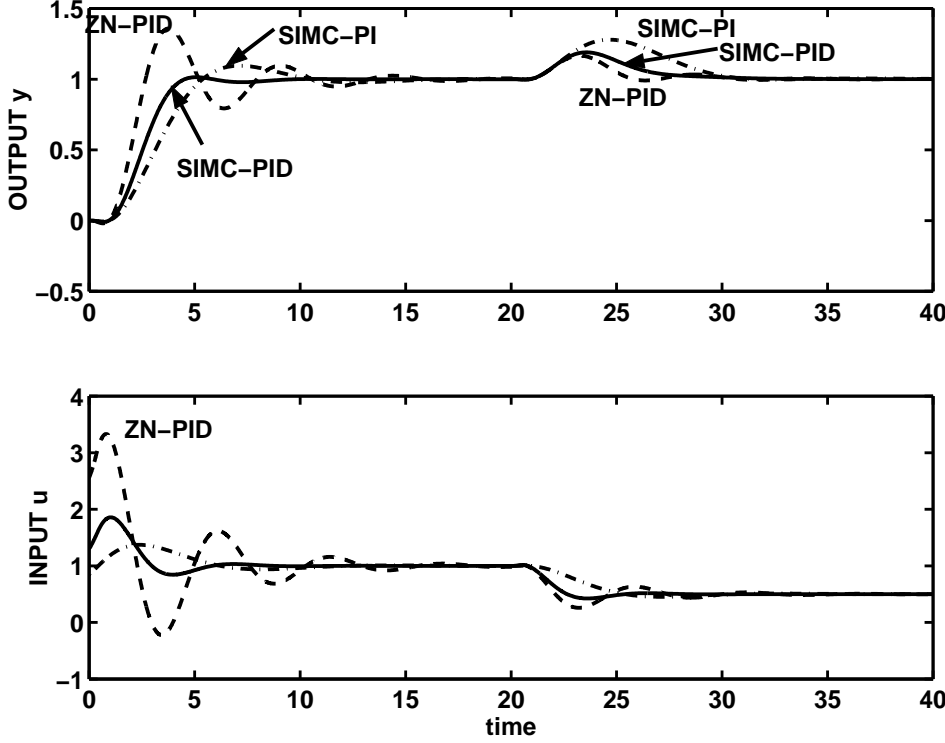
Figure 8: Example 2. Responses for process (49) with tunings from Table 4
