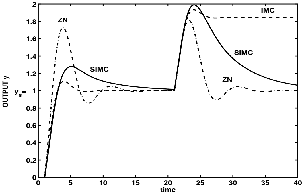
Figure 5: Responses for PI-control of integrating process, g(s) = e^{-s}/s , with settings from Table 5 Setpoint change at t = 0 ; load disturbance of magnitude 0.5 at t = 20 .
