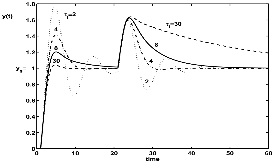
Figure 3: Effect of changing the integral time \tau_I for PI-control of “almost integrating” process g(s) = e^{-s}/(30s + 1) with K_c = 15 .
