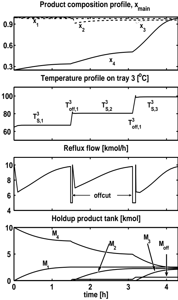
Figure 3: Product composition profile, controlled temperature, reflux flow and holdups of products for conventional batch distillation
