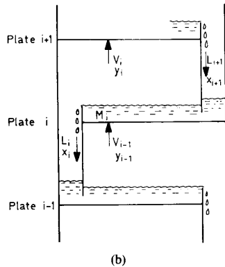
Fig. 2. Two-product distillation column. Details of the flows and holdups on a plate are shown.
