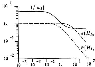
Fig. 10. LV -configuration. RS bounds.
