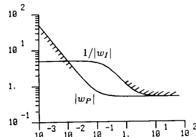
Fig. 8. Multivariable loop shaping.
