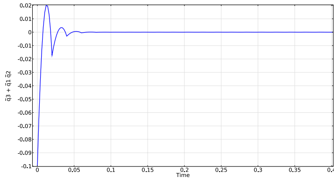
Fig. 7. Plot of \bar{q}_3 + \bar{q}_1\bar{q}_2 with \alpha = 1 and \varepsilon = 10^{-20} under FICK constraint. Initial conditions are \bar{q}_1 = 0 , \bar{q}_2 = 0 , \bar{q}_3 = -0.1 and final conditions \bar{q}_1 = 1 , \bar{q}_2 = 0 , \bar{q}_3 = 0 . Initial and final conditions on \omega are chosen as zero.
