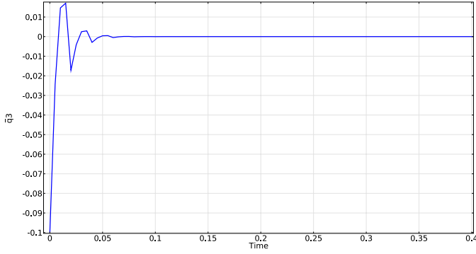
Fig. 4. Plot of \bar{q}_3 with \varepsilon = 10^{-18} and \alpha = 1 when Listing's law is imposed as a constraint. Initial conditions are \bar{q}_1 = 0, \bar{q}_2 = 0, \bar{q}_3 = -0.1 and final conditions are \bar{q}_1 = 1, \bar{q}_2 = 0, \bar{q}_3 = 0 . Initial and final conditions on \omega are chosen as zero.
