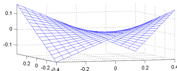
Fig. 1. Donders' surface corresponding to the Fick gimbal has been sketched using the scaled co-ordinates \bar{q}_i = \frac{q_i}{q_0} for i = 1, 2, 3 . The coordinate \bar{q}_3 along the vertical line shows the nonzero torsion.
