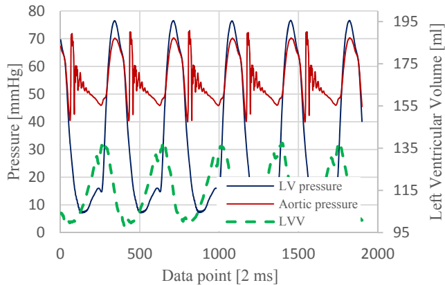
Fig. 7 Unfiltered LVP and AoP curves using water, together with LVV of a simulated pathological heart; HR = 81, SV = 38 ml, SBP/DBP = 70/50 mmHg, LVEF 28%
