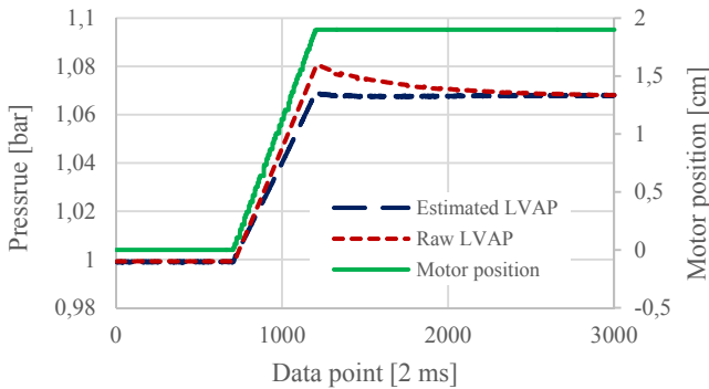
Fig. 5. Response of raw and estimated LVAP to the piston's position change.
