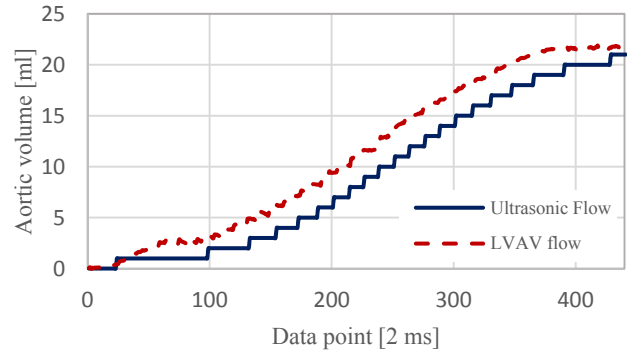
Fig. 6. Comparison of unfiltered measurements using the ultrasonic and newly developed LVAV flow sensing principle.
