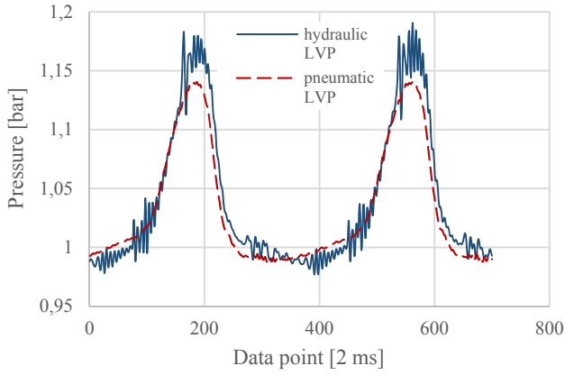
Fig. 4. LVP response with hydraulic and pneumatic actuation.
