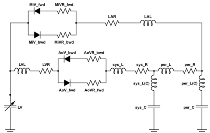
Fig. 1. Lumped parameter model of the mock circulation.
