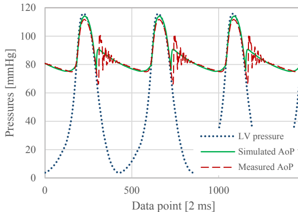
Fig. 2. Simulated vs. measured aortic pressure with the same LV pressure reference. Lumped model parameters: LVL = 2.1 \cdot 10^5 H , LVR = 1.9 \cdot 10^4 \Omega , sys\_L = 3.7 \cdot 10^5 H , sys\_R = 4.7 \cdot 10^6 \Omega , sys\_C = 1.7 \cdot 10^{-8} F , per\_L = 5.1 \cdot 10^5 H , per\_R = 7.5 \cdot 10^7 \Omega , per\_C = 1.8 \cdot 10^{-6} F , LAL = 10^6 H , LAR = 3.9 \cdot 10^4 \Omega .
