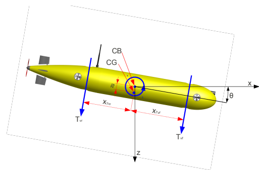
Fig. 2. Schematic of the location of the thruster force vectors, moment arms, center of gravity and buoyancy and the axis system, where the pitch angle is -10^\circ .
