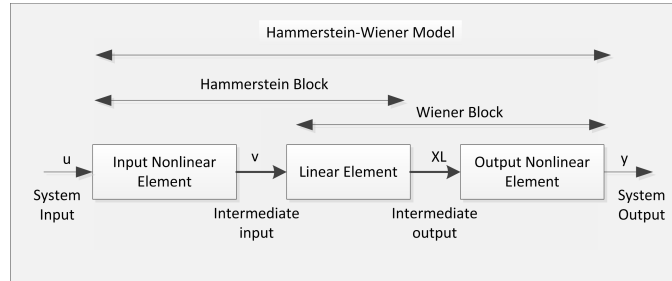
Fig. 1. Hammerstein-Wiener block structure
