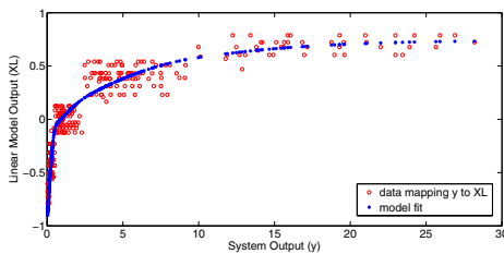
(b) Quadratic B-Spline
