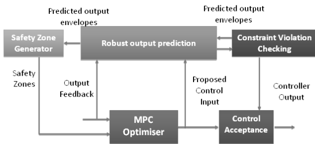
Fig. 5. Structure of RFMPC with iterative safety zones.
