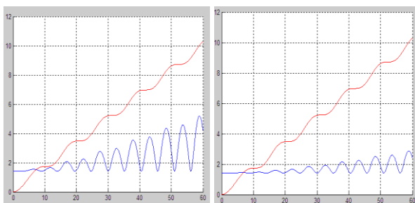
Fig. 14 – Time behaviour of the norm of e in meters (blue) and the norm of X in hundreds of meters (red)
