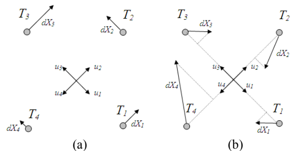
Fig. 4 – Scenarios of null contribution provided by b_i terms. a) every b_i term is null, as every dX_i vector is orthogonal to its corresponding u_i ; b) b_i terms are not null but their resulting contribution to error vector e is null
