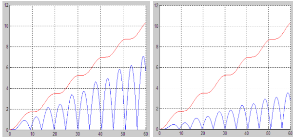
Fig. 10 – Time behaviour of the norm of e in meters (blue) and the norm of X in hundreds of meters (red)
