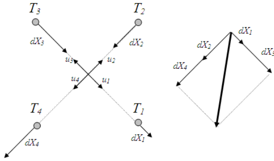
Fig. 5 – Scenario of non null contribution provided by b_i terms. The resulting vector is in bold.
