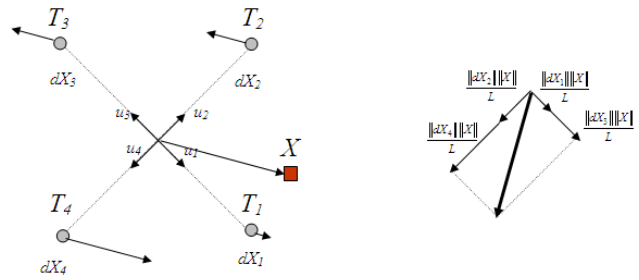
Fig. 7 – Worst-case scenario for the error contribution provided by c_i terms. The resulting vector is in bold..
