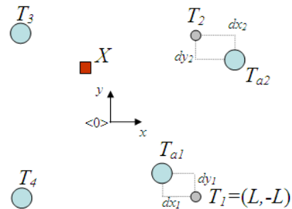
Fig. 2 –Nominal positions (grey) and actual positions (cyan) of transponders in the presence of displacements
