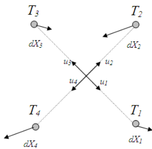
Fig. 6 – Null resulting contribution to the error e provided by c_i terms
