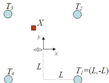
Fig. 1 – squared configuration of transponders
