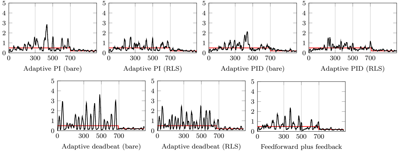
Fig. 1. Average latency (black) and corresponding setpoint (red) for the experiment varying application popularity and requirements.
