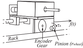
Figure 1: Cart System
