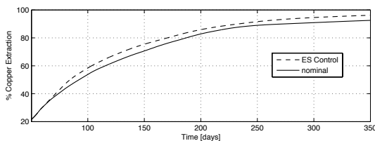
Fig. 7. Total copper extraction [%] for ESC to maximise concentration of [CuSO 4 ] using aeration
