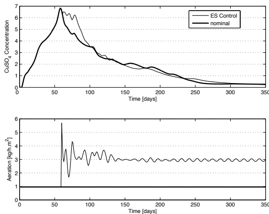
Fig. 6. ESC applied to maximise concentration of [CuSO 4 ] (top) by manipulating aeration (bottom)
