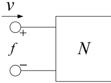
Fig. 1. One-port network system representing components. The conjugate variables that define power flow in such a network system are discrete-time values, and the analysis was confined to systems having a sampling rate substantially faster than the dynamics of the system. Thus, we could easily “instrument” one or more blocks in the system with the following “Passivity Observer,” (PO) for a one-port network to check the passivity (1).
