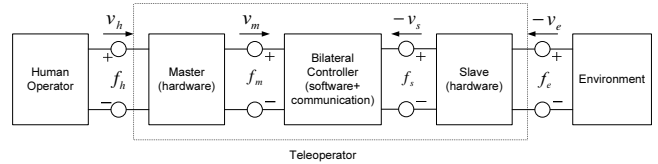
Fig. 3. Block diagram of a complete teleoperation system.
