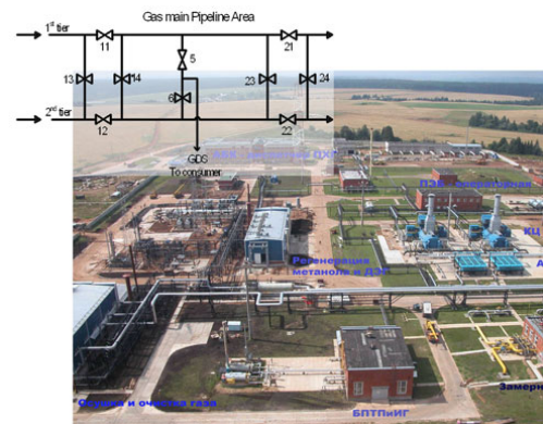
Figure 1 Line area of gas main pipeline
