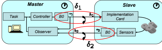
Fig. 1. Structure of the remote system under time-varying delays, samplings and packet loss.
