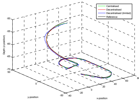
Fig 1: A 3-D view of a performance comparison between the centralised and decentralised MPC
