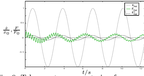
Fig. 9. Teleoperator encountering free space
