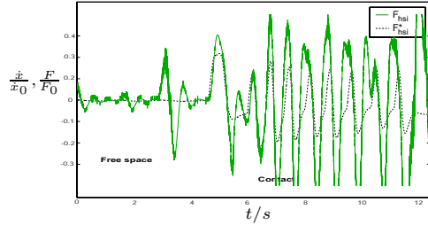
Fig. 10. Telepresence in free space and contact
