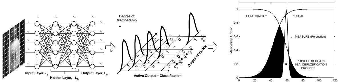
Fig. 5 Decision in fuzzy environment with constraint imposed by cognitive process of visual perception.
