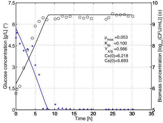
Fig. 1. Evolution of the glucose (*) and biomass (o) concentration measurements in function of time and the model predicted profiles (–) with the corresponding identified values for the model parameters and initial conditions.
