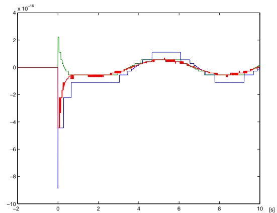
Fig. 5. The error of the estimation of the state variable number 3-5
