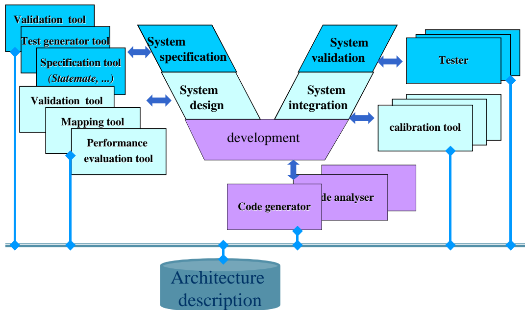
figure 1 Development process activities
