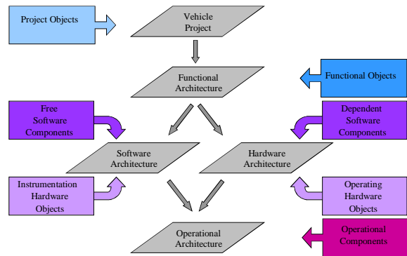
figure 2 Architectures and main classes
