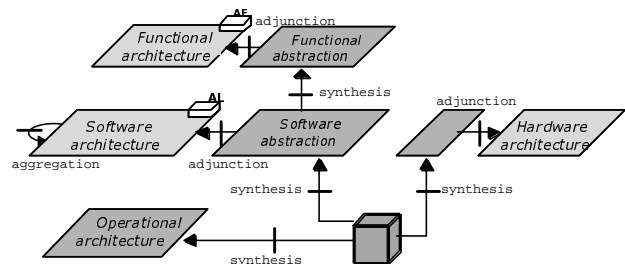
Fig. 5. How to add a sub-contracted element
