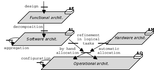
figure 2 Fig. 3. Ex-nihilo building process
