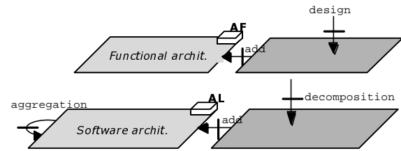
figure 3 Fig. 4. Construction of a new architectural element
