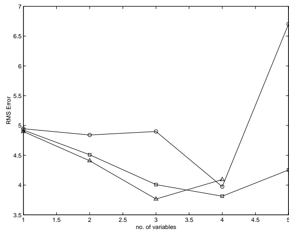
Fig. 5. J_{TS} versus the number of input variables for each model using variables selected by the first method (squares), the second (triangles) and the third method (circles).
