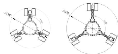
Fig. 3. The diameter transmission range of the Smart-Spider can be from 450 mm to 575 mm
