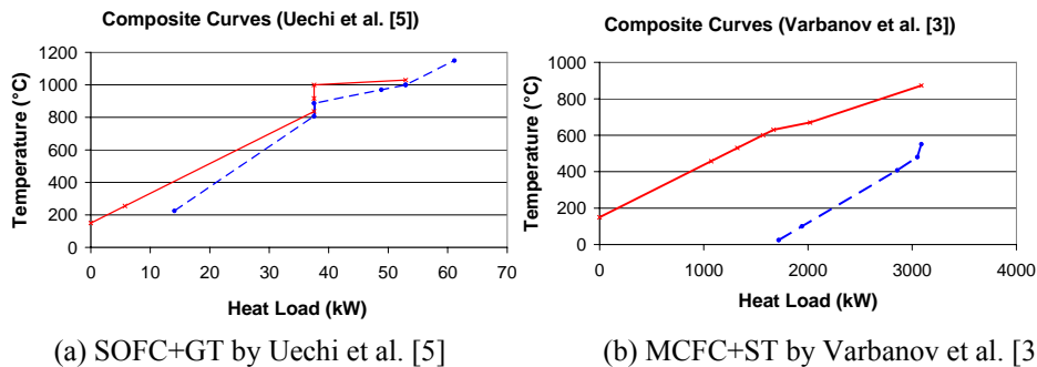
Fig 2. Composite curves (CC) of FC integration
