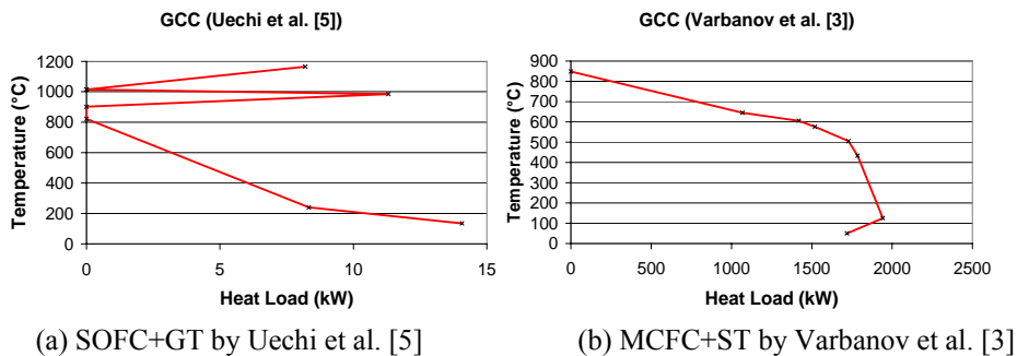
Fig 3. Grand Composite Curves (GCC) of FC integration
