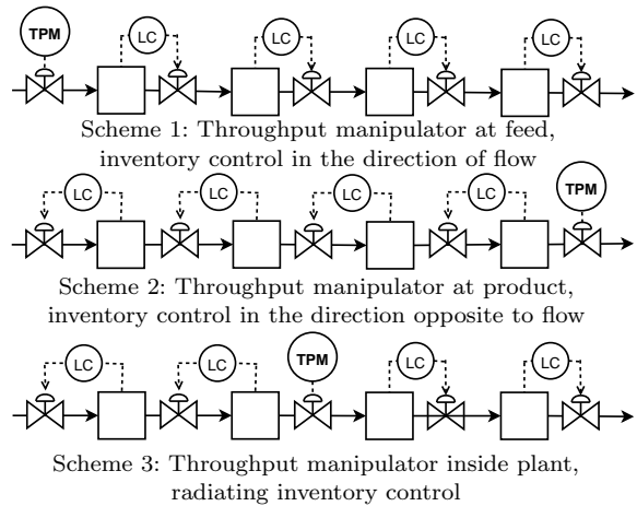
Fig. 1. Basic schemes for inventory control
