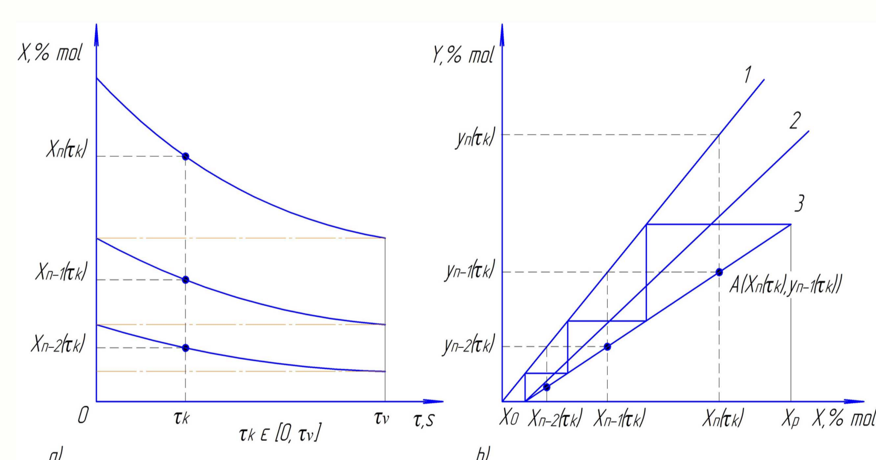
Figure 1. The methodology of construction of the perfect displacement mode operating line is as follows: a) Temporary concentration profiles in liquid; b) Depicting of the perfect displacement operating line in X-Y coordinates; 1 - equilibrium line; 2 - perfect mixing operating line; 3 - perfect displacement operating line.
