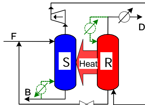
Figure 8. The HIDiC principle
