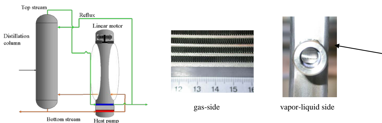
Figure 6. The electrically driven TA heat pump (left) and heat exchanger details (middle and right)
