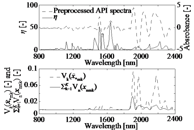
Figure 2. Wavelength selection index \eta and preprocessed API spectra and (bottom)
