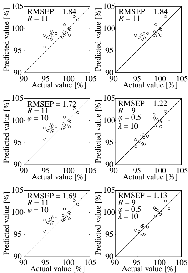
Figure 1. Results of model validation. (left-top) case 1: PLS with all wavelengths, (right-top) case 2: PLS with the proposed wavelengths, (middle-top) case 3: LW-PLS 1 with all wavelengths, (middle-top) case 4: LW-PLS 1 with the proposed wavelengths, (left-bottom) case 5: LW-PLS 2 with all wavelengths, and (right-bottom) case 6: LW-PLS 2 with the proposed wavelengths.
