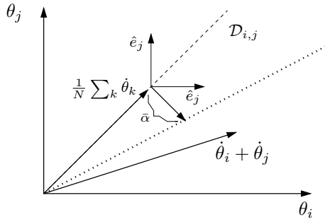
Fig. 1. Geometric interpretation of desynchronization
