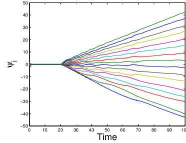
Fig. 3. Evolution of the grounded dynamics of (17) for large natural frequencies when a proportional mean-field feedback with gain \gamma = -k_0 is switched on at time t = 20 .
