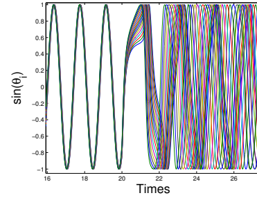
Fig. 2. Evolution of the phases of (17) for large natural frequencies when a proportional mean-field feedback with gain \gamma = -2k_0 is switched on at time t = 20 . The mean-field feedback induces desynchronization.
