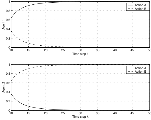
Fig. 1. Typical response of \tilde{\mathcal{L}}_{R-I}^\lambda on the Typewriter Game of Table I when \nu = 0.78 .
