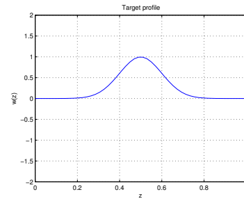
Fig. 1: Desired steady state target profile(reference profile), w_{ref}(z) \in D(A)
