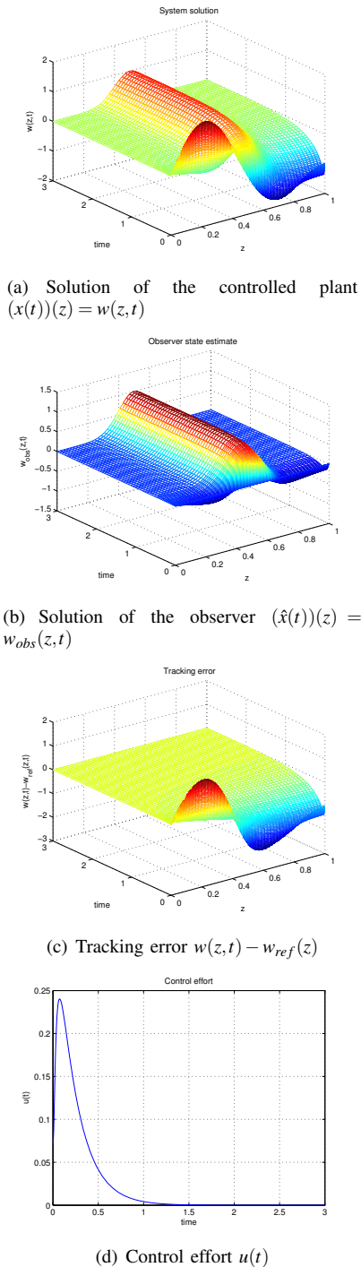
Fig. 2: System and Observer solutions
