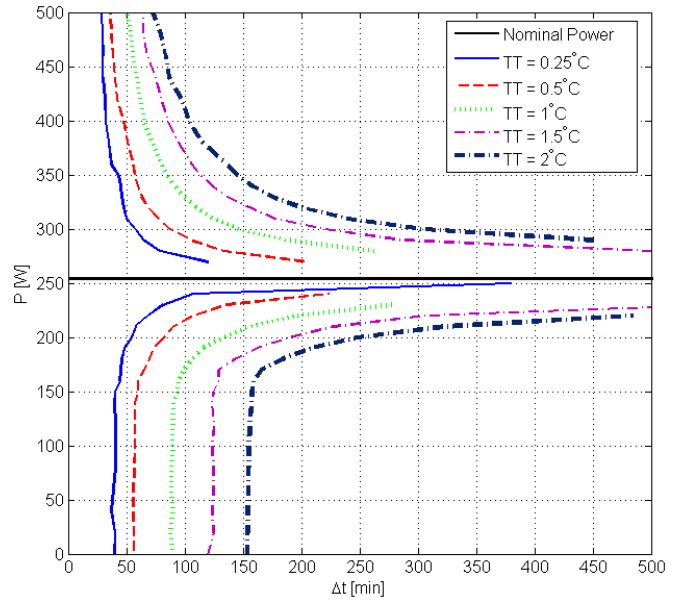
Fig. 4. Power setpoint generation assistant chart for a 54 m 2 flat, containing several thermal tolerance (TT) levels
