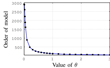
Fig. 5. Order of resultant models versus values of \theta .
