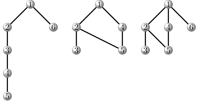
Fig. 1. Examples of Proposition 3
