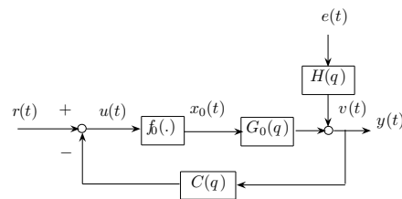
Fig. 1. Closed-loop Hammerstein system.
