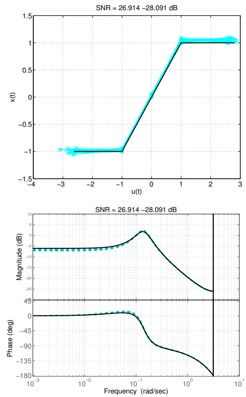
Fig. 4. Case 2 : The plot of the identified static nonlinearity function (top figure). The Bode plot of the identified linear dynamic system (bottom figure). The black solid line indicates the real Hammerstein system. The (colored) dashed lines indicate estimated systems by using twenty different sets of data. The SNR of each data set spans the values between 26.914 and 28.091dB.
