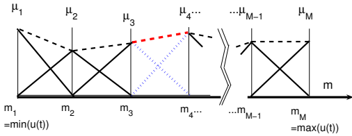
Fig. 2. Triangle basis functions.
