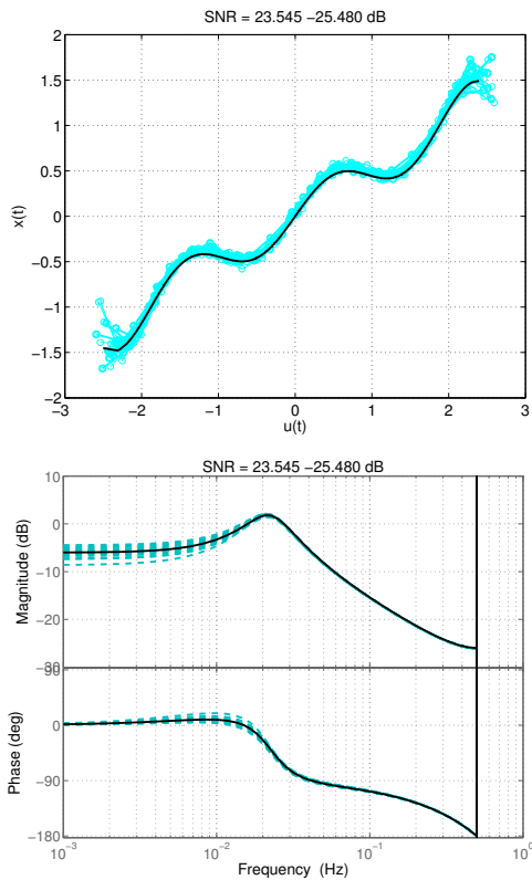
Fig. 3. Case 1 : The plot of the identified static nonlinearity function (top figure). The Bode plot of the identified linear dynamic system (bottom figure). The black solid line indicates the real Hammerstein system. The (colored) dashed lines indicate estimated systems by using twenty different sets of data. The SNR of each data set spans the values between 23.545 and 25.480dB.
