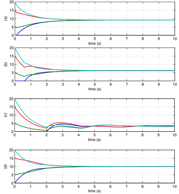
Fig. 1. Simulation results for A_0 and Corollary 1 type with \tau = 0.1 (a), \tau = 0.6 (b) and \tau = 2 (c) and Corollary 2 with \tau = 0.6 (d)
