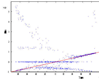
Fig. 4. Estimates of \theta via EKF (large initial variance).
