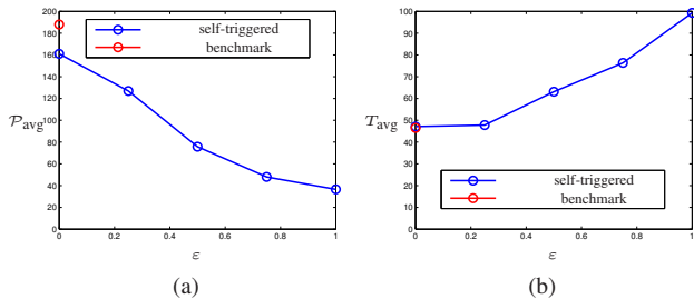
Fig. 5. Plots of the average (a) communication power consumption \mathcal{P}_{\text{avg}} and (b) timesteps to convergence T_{\text{avg}} over 20 simulations for varying \varepsilon .
