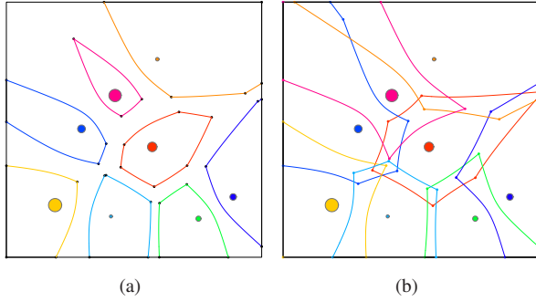
Fig. 2. Guaranteed Voronoi (a) and dual guaranteed Voronoi (b) diagrams. belongs to a set of the form
