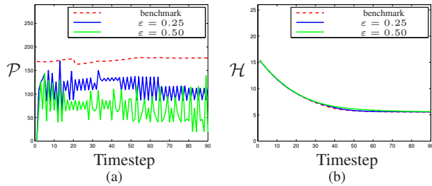
Fig. 4. Plots of (a) the communication power \mathcal{P} used by the network and (b) the value of \mathcal{H} in each timestep comparing three different executions.
