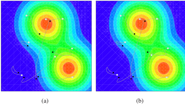
Fig. 3. Network trajectories of (a) the benchmark case and (b) the self-triggered centroid algorithm with \varepsilon = 0.25 . The black and grey dots correspond to the initial and final agent positions, respectively.
