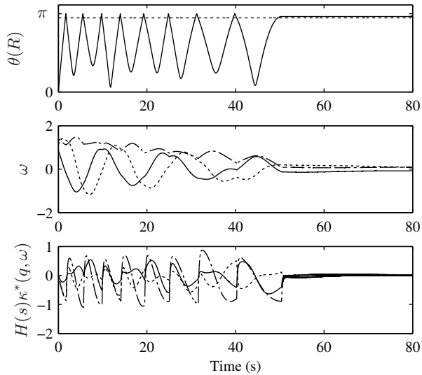
Fig. 1. Effects of malicious disturbance on inconsistent quaternion-based feedback composed with a memoryless lifting map. The manifold \mathcal{U}(\pi, \mathbb{S}^2) \times \{0\} \subset \text{SO}(3) \times \mathbb{R}^3 is stabilized. Top: solid line is \theta(R) = \cos^{-1}((\text{trace}(R) - 1)/2) , dashed line is \pi - \delta . Middle: solid line is \omega_1 , dashed line is \omega_2 , dash-dot line is \omega_3 . Bottom: shows a filtered version of \tau = \kappa^*(q, \omega) defined in (19). Solid line is \tau_1 , dashed line is \tau_2 , dash-dot line is \tau_3 .
