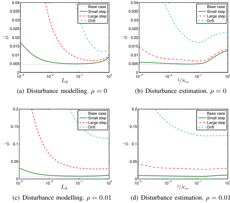
Fig. 1. Closed loop performance for the four simulation scenarios using both MPC implementations with \rho \in \{0, 0.01\} . The performance is plotted as function of the disturbance state estimator gain L_d for the disturbance model approach and the inverse of the equivalent horizon N_\infty for the disturbance estimation approach with time varying forgetting.
