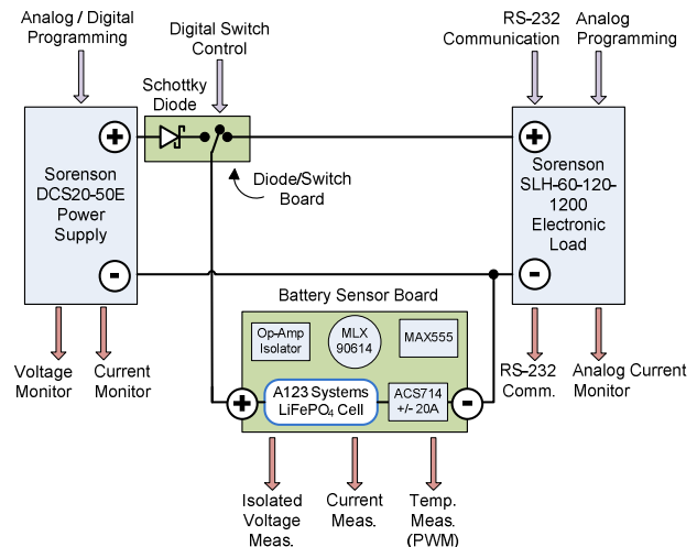
Fig. 2. Schematic of Experimental Battery Tester
