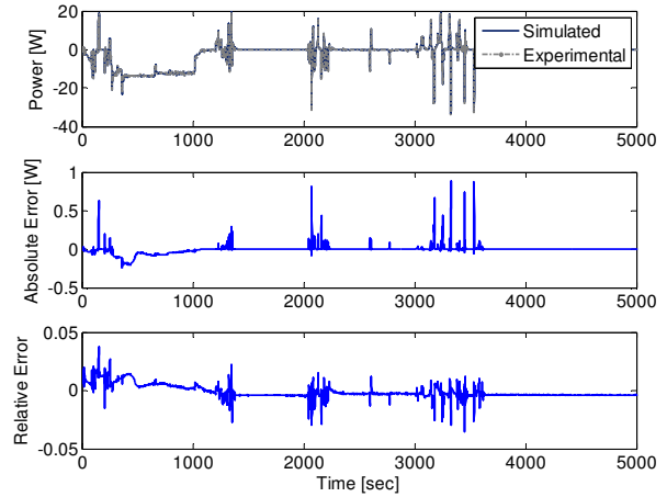
Fig. 6. Power Response for Naturalistic2 .
