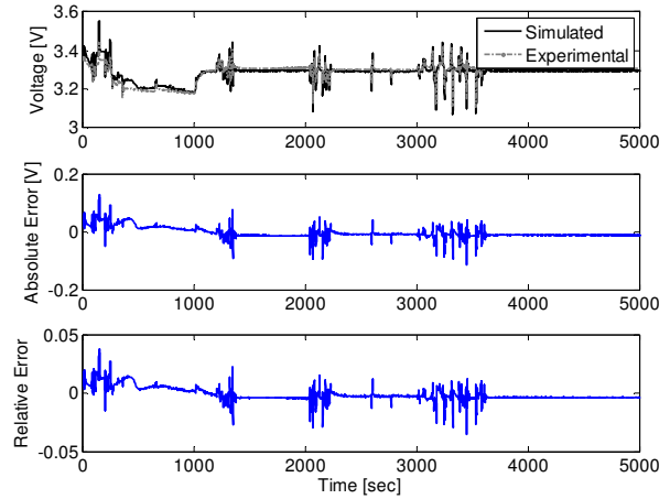
Fig. 5. Voltage Response for Naturalistic2 .
