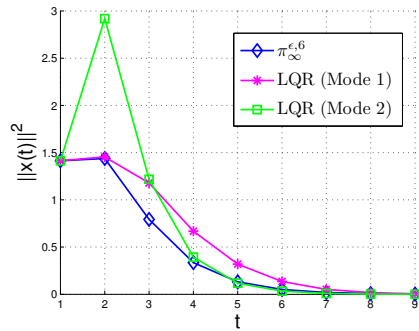
Fig. 4. Euclidean norms of the closed-loop trajectories with initial condition x(0) = [1, 1]^T driven by different feedback policies.
