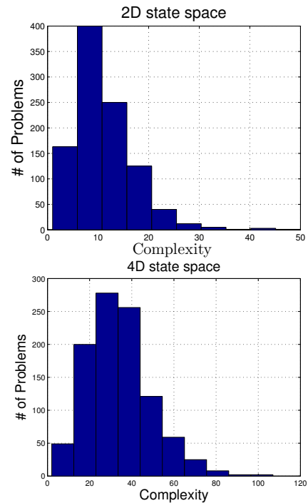
Fig. 5. Complexity distributions of the random examples.
