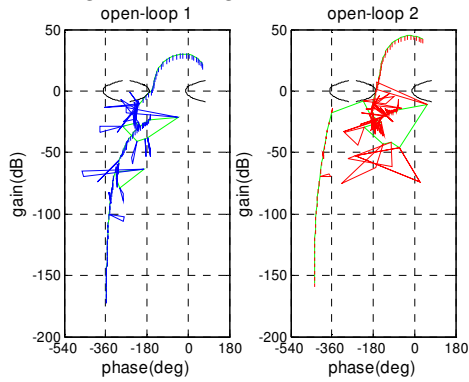
Fig.5. Nichols loci for \beta_{01}(s) and \beta_{02}(s)
