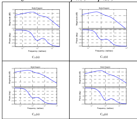
Fig.6. Bode diagrams of the terms of the controller
