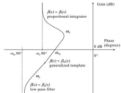
Fig.2. Different parts of the open-loop Nichols locus
