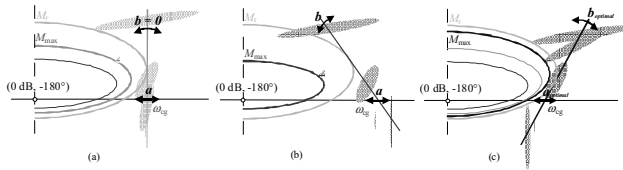
Fig.3. Optimal open-loop Nichols locus to position the uncertainty domains
