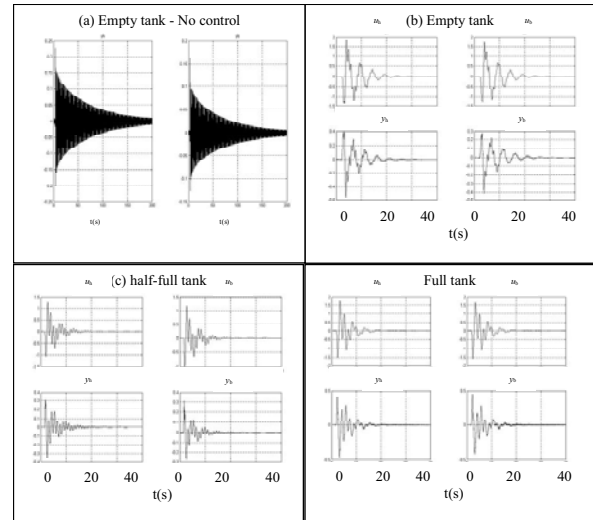
Fig.7. Response to a perturbation
