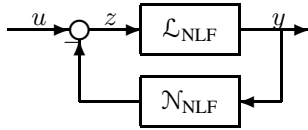
Fig. 3. Nonlinear Feedback Model
