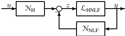
Fig. 4. Hammerstein Nonlinear Feedback Model
